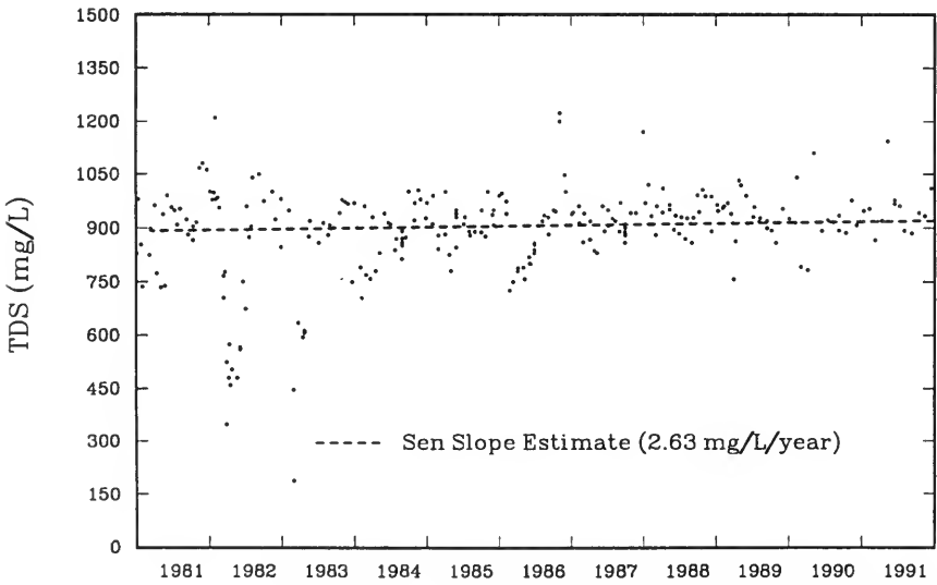
Figure 3.6 Sen Slope Estimate for TDS at East Poplar River at the International Boundary.
